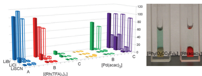
Figure 3. a) Initial hits from visual colorimetric ISES are ranked spectrophotometrically ( Abs_{405} in mAbs\ min^{-1} ; A, B, and C are substrates 3 , 7 , and 8 , respectively; see the Supporting Information for experimental details). b) An example of the cuvette ISES experiment. The ABTS indicator shows turnover with Rh^{II} perfluorobutyrate, whereas the highly colored Rh^{III} catalyst fails.
